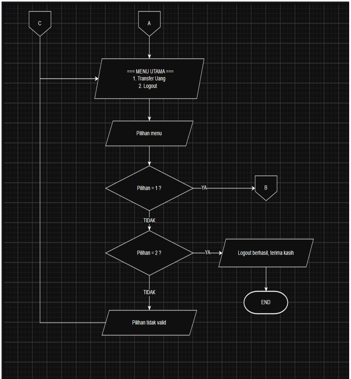
Gambar 1.2 Flowchart page 2
