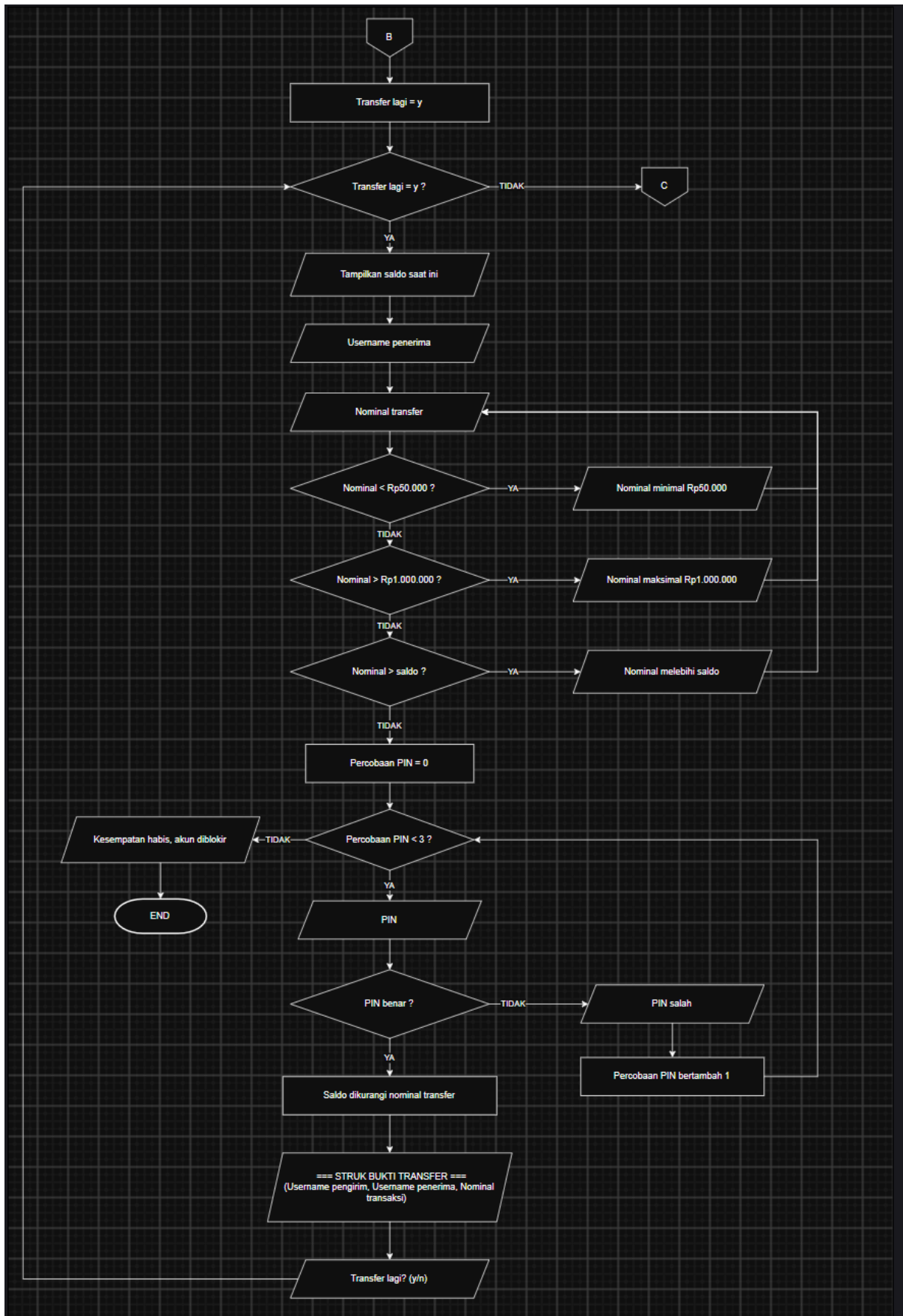
Gambar 1.3 Flowchart page 3
